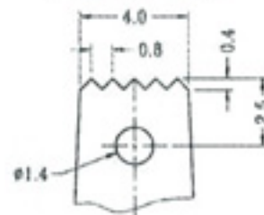
KNOB DETAIL (5:1)
